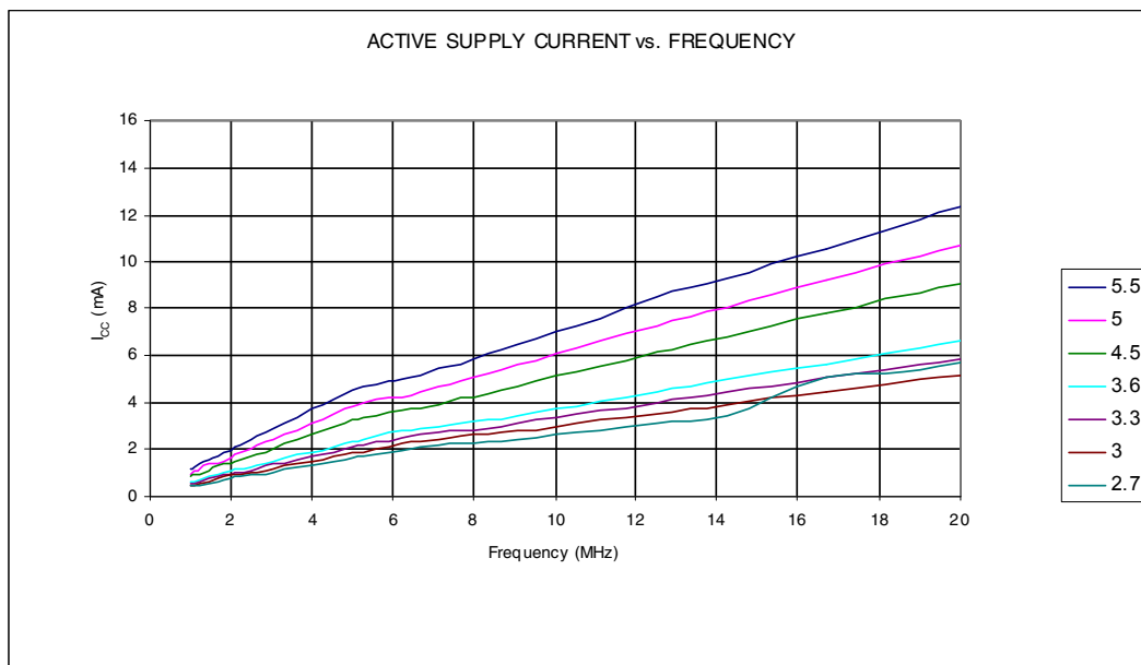
Figure 29-1. Active Supply Current vs. Frequency.
