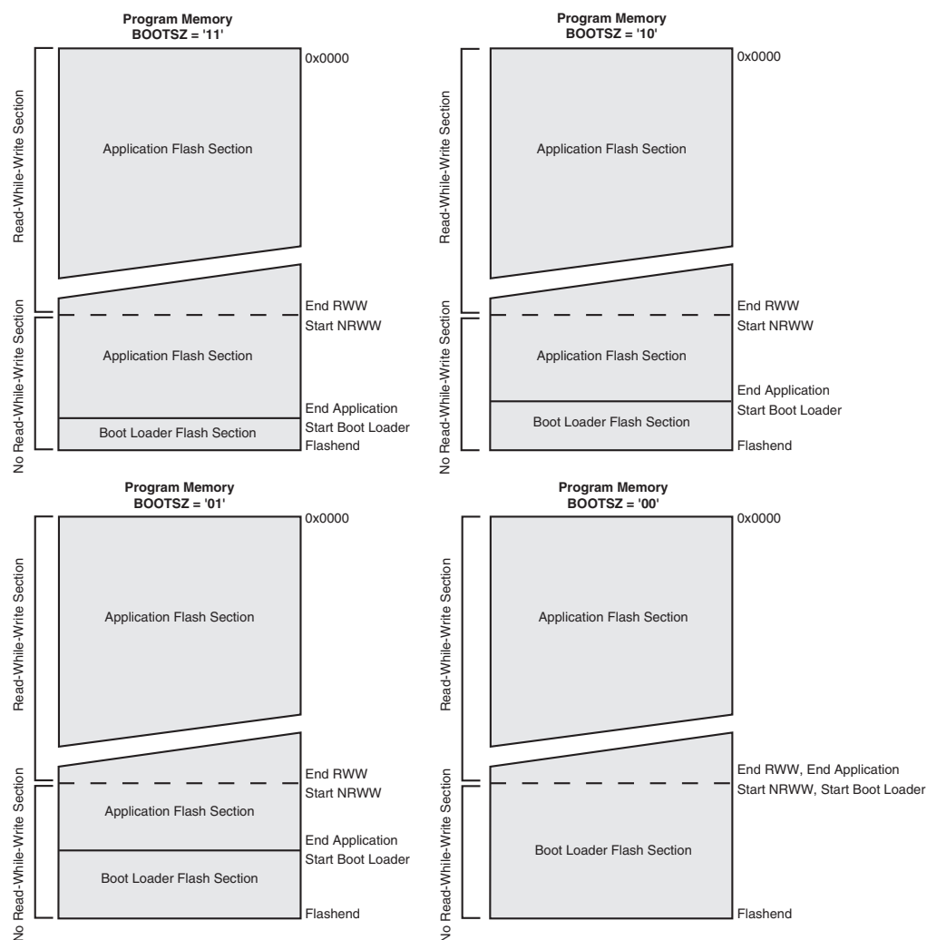
Figure 26-2. Memory Sections
