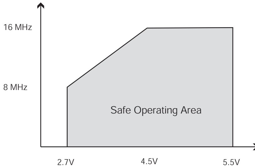
Figure 28-1. Maximum Frequency
