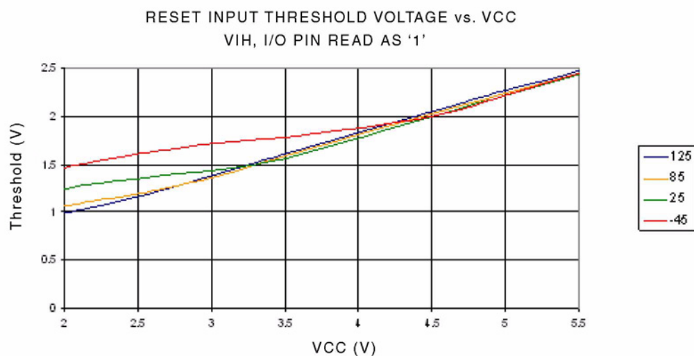
Figure 29-13. Reset Input Threshold Voltage vs. V_{CC} ( V_{IH} , I/O Pin read as '1').
