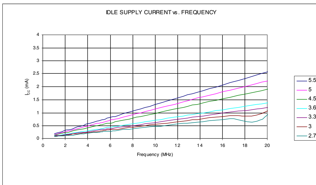
Figure 29-2. Idle Supply Current vs. Frequency..
