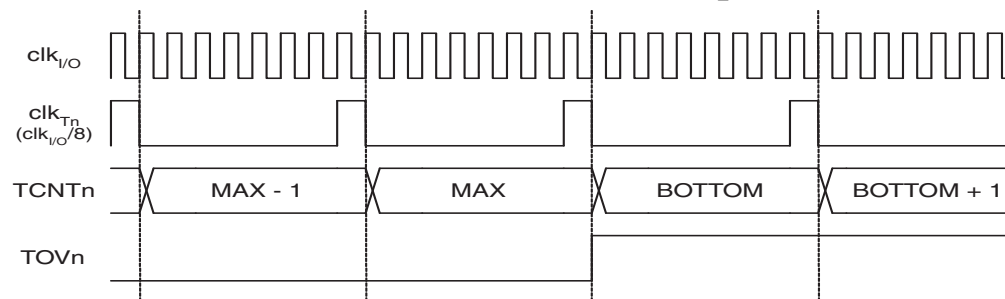
Figure 17-9. Timer/Counter Timing Diagram, with Prescaler ( f_{\text{clk}_{I/O}}/8 )
