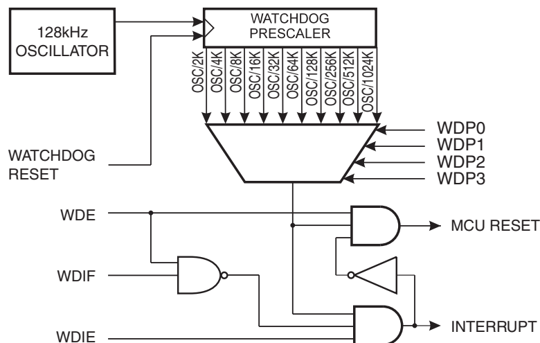
Figure 10-7. Watchdog Timer
