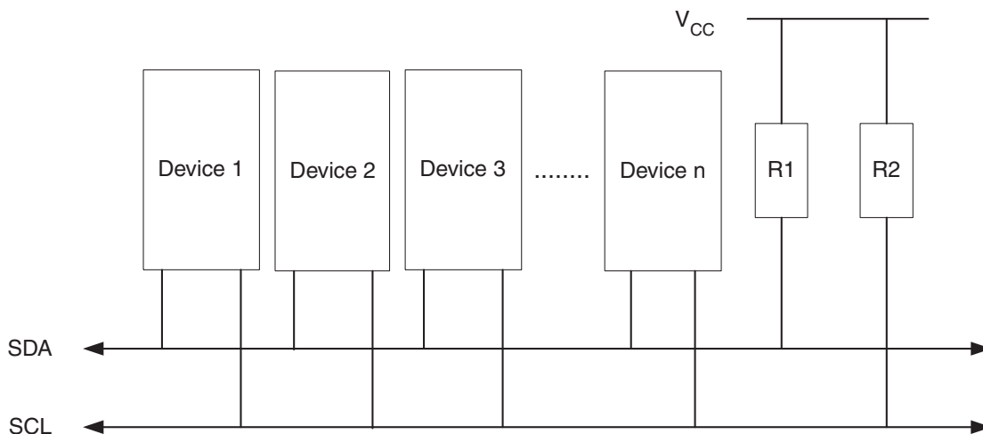
Figure 21-1. TWI Bus Interconnection
